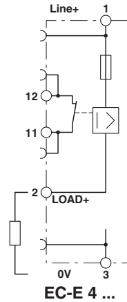
Circuit diagram
